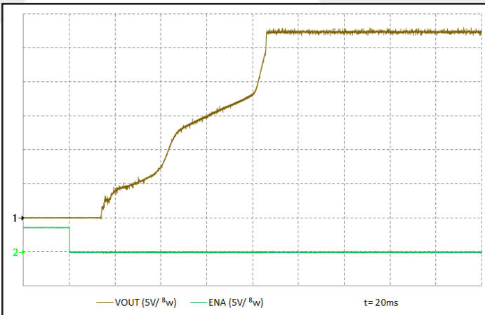
Figure 9: Turn-on transient at half resistive load and 100 uF output capacitance initiated by ENA. Input voltage pre-applied. Ch 1: Vout (5 V/div). Ch 2: ENA (5 V/div). Timescale: 20.0ms/div. Bandwidth: 20 Mhz.
