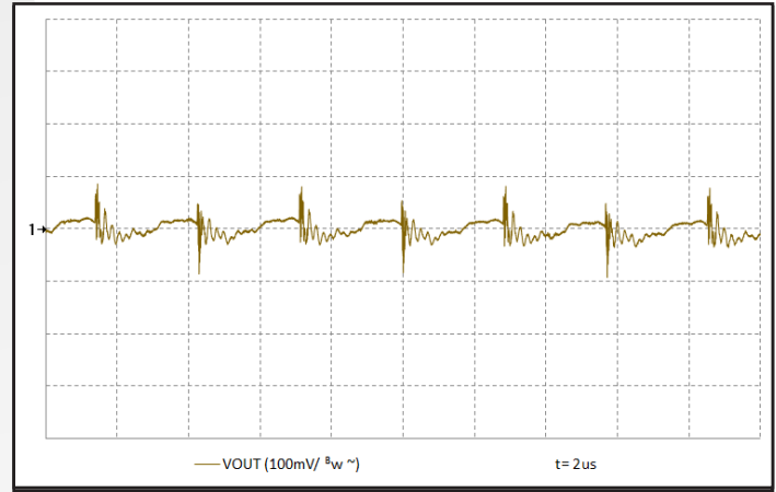
Figure 16: Output voltage ripple, V_{out} , at nominal input voltage and full load, 470uF output capacitance (100 mV/div). Bandwidth: 20MHz. Timescale: 2.00 \mu s/div. See Figure 12.
