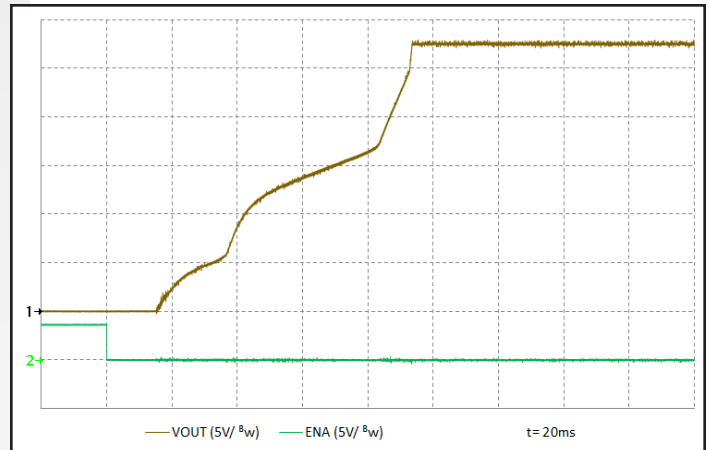
Figure 10: Turn-on transient at half resistive load and 9 mF output capacitance initiated by ENA. Input voltage pre-applied. Ch 1: Vout (5 V/div). Ch 2: ENA (5 V/div). Timescale: 20.0ms/div. Bandwidth: 20 Mhz.
