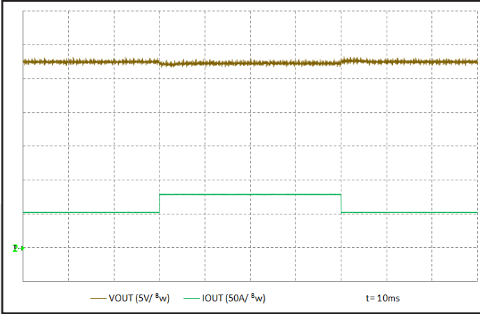
Figure 13: Output voltage response to step-change in load current 50%-75%-50% of I_{out(max)} , 470uF output capacitance. Ch 1: V_{out} (5 V/div) Ch 2: I_{out} (50A/div). Bandwidth: 20 MHz. Timescale: 10.0ms/div.
