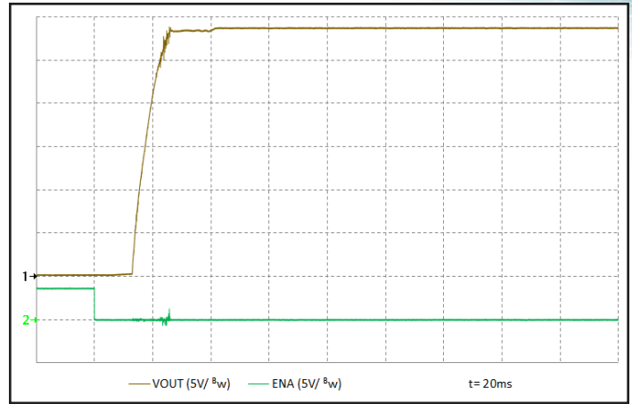
Figure 8: Turn-on transient at no load and 470uF output capacitance initiated by ENA. Input voltage pre-applied. Ch 1: Vout (5 V/div). Ch 2: ENA (5 V/div). Timescale: 20.0ms/div. Bandwidth: 20Mhz.
