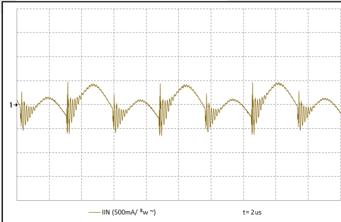
Figure 15: Input terminal ripple, i_c , at full load and nominal input voltage with 10 \mu H source impedance and 110 \mu F electrolytic capacitor (500 mA/div). Bandwidth: 20 MHz. Timescale: 2.00 \mu s/div. See Figure 12.
