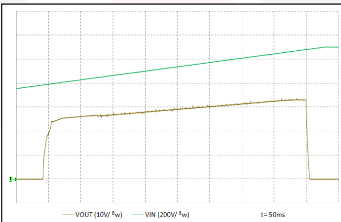
Figure 11: Under-Voltage Lockout and Over-Voltage Shutdown behavior as a function of V_{in} . ENA previously enabled. 100uF output capacitance Ch 1: Vout (10 V/div). Ch 2: Vin (200 V/div). Timescale: 50.0ms/div. Bandwidth: 20 Mhz.
