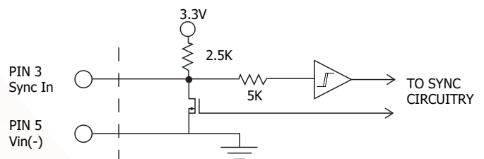
Figure C: Equivalent circuit looking into the Sync In pin with respect to the Vin(-) (input return) pin.
